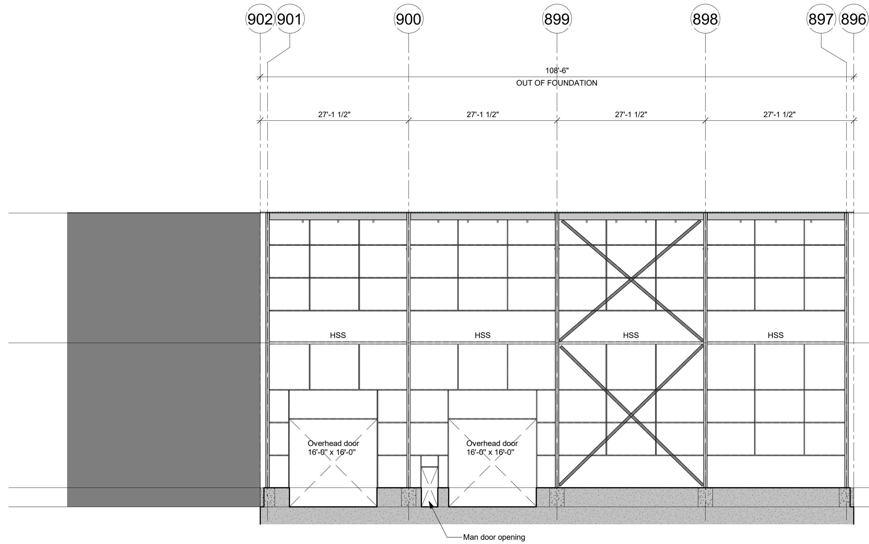
ELEVATION LINE BBB (WEST) 3/32" = 1'-0"
