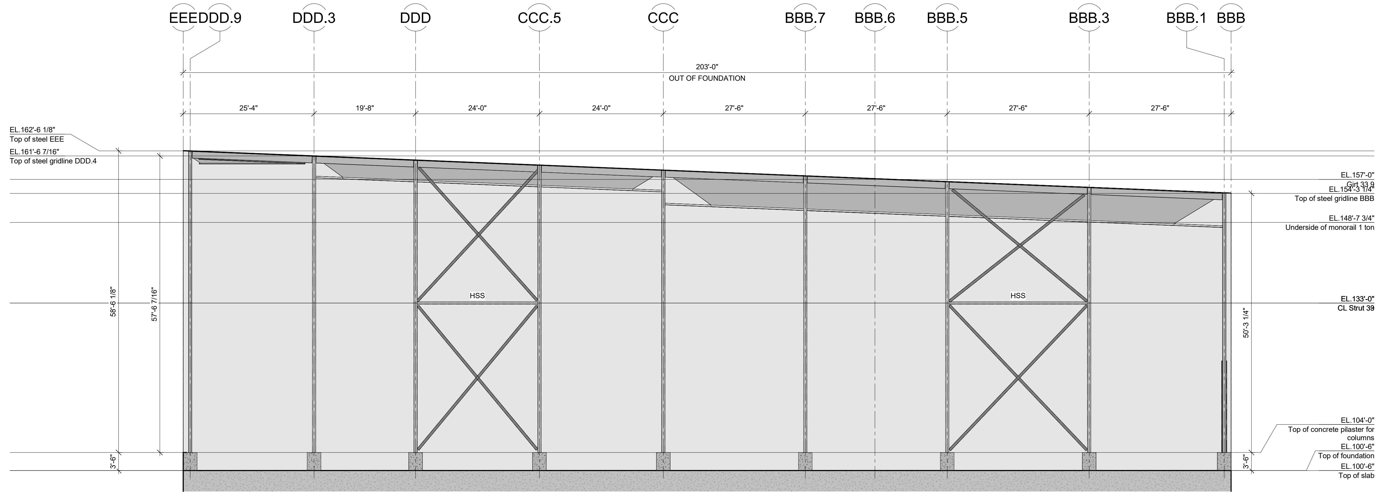
ELEVATION LINE 907 & 910 (NORTH) 3/32" = 1'-0"
