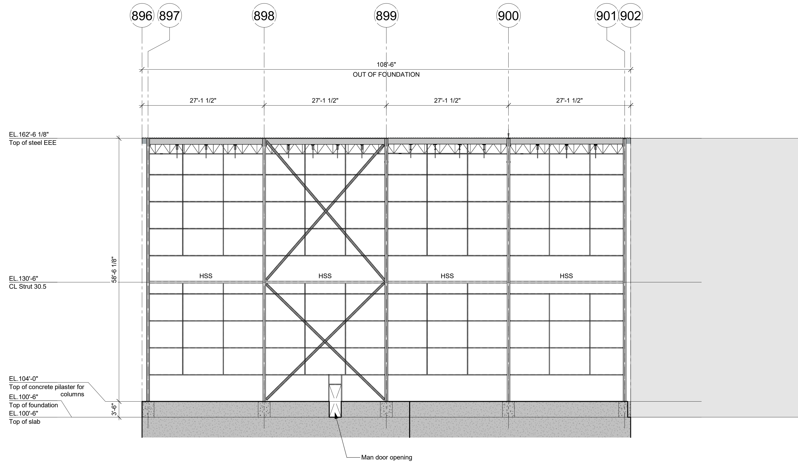
ELEVATION LINE EEE (EAST) 3/32" = 1'-0"
