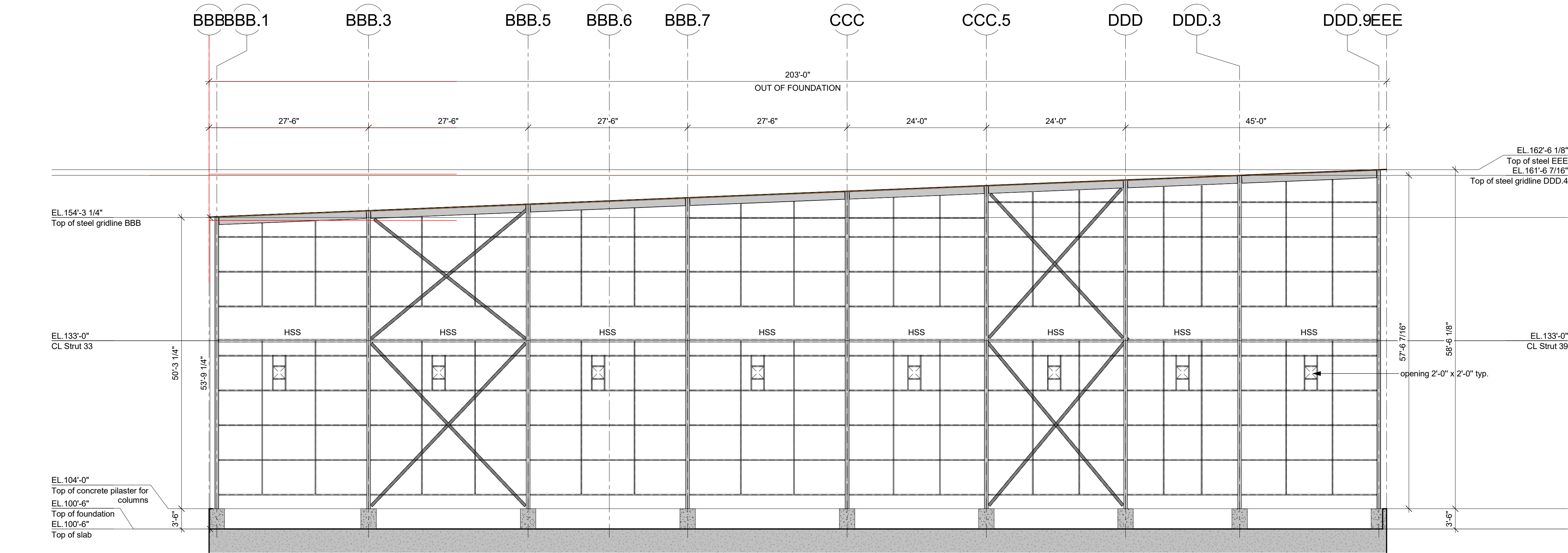
ELEVATION LINE 902 (SOUTH) 3/32" = 1'-0"
